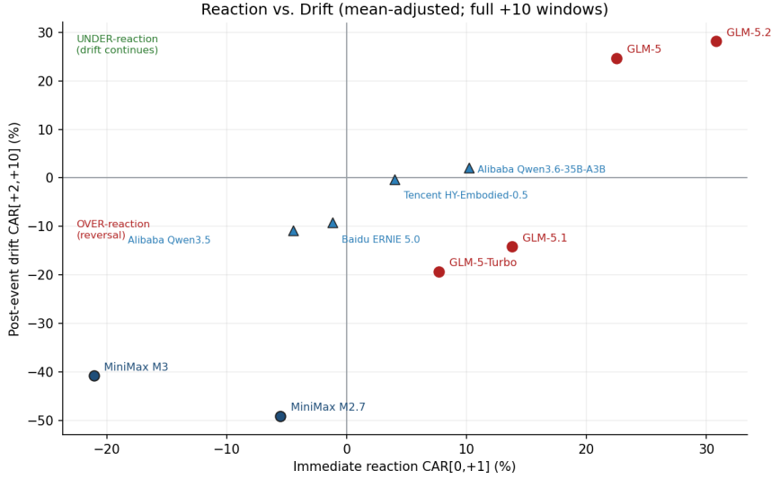
Figure 10: Reaction versus drift. SOTA leaps sit in the under-reaction quadrant; incremental upgrades in the over-reaction quadrant. Triangle markers show large-tech AI comparators.
